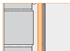
12.1 Schluter®-KERDI-BOARD
