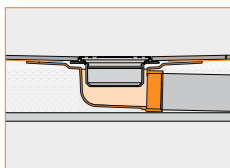
8.2 Schluter®-KERDI-DRAIN-H
